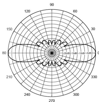
Diagrama Vertical
