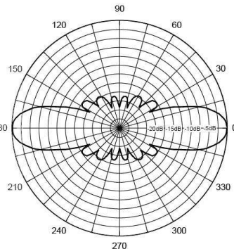
Diagrama Vertical
